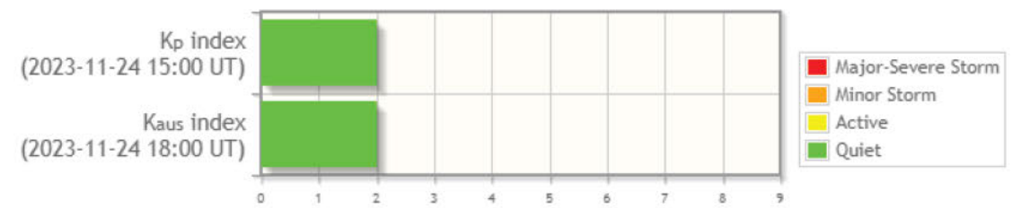
Latest estimated 3-hour K-Index data
